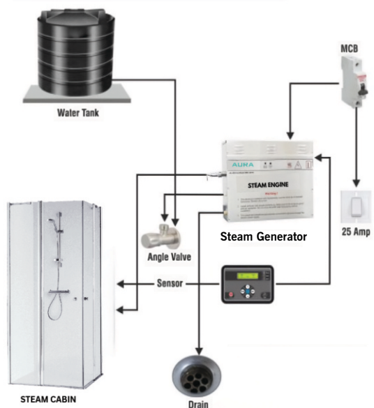
INSTALLATION DIAGRAM
